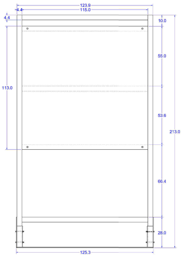
Vista Frontal
